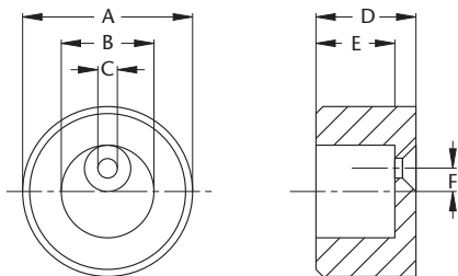
Figure 63: HEKO bearing bush
