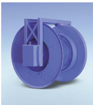
Figure 68: Pre-assembled HEKO Return and Tensioning unit, complete with segmented rims and spacer bars.
