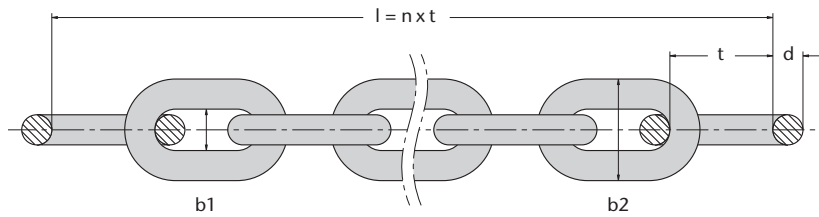
Figure 7: Dimensions for round link chains
