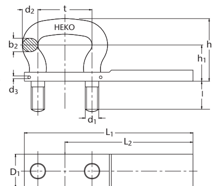
Figure 15: HEKO shackle type TS-L
