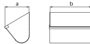
Figure 36: Bucket execution B – with front re-enforcing rim
