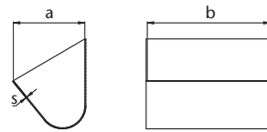
Figure 35: Bucket execution A – without re-enforcing rim
