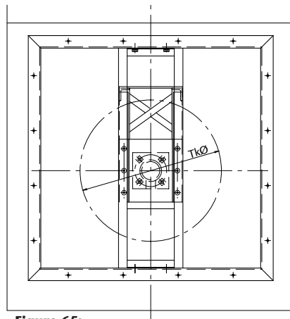
Figure 65: Drawing of a return and tensioning unit. Picture right corner: Assembly of a HEKO return unit.
