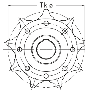
HEKO chain wheel type RLA-R with symmetric teeth, reversible operation
