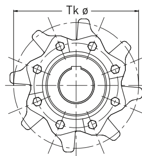
HEKO chain wheel type RLA for forged link chains model 69226
