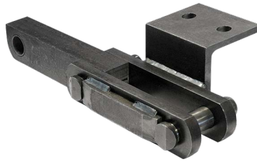
Double-strand block link chain with welded attachment angle at the outer link and wear plate
