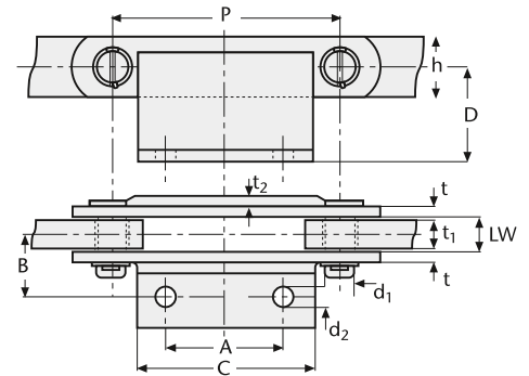
Double-strand block link chain with welded attachment angle at the outer link and wear plate
